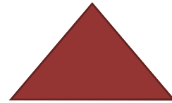
Triangle
