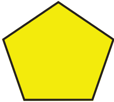
Pentagon
