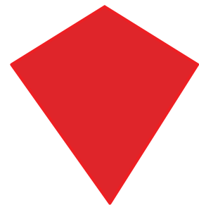
Kite
