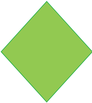
Diamond
