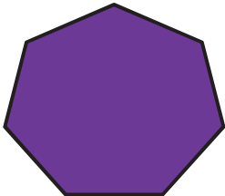
Heptagon
