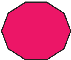
Decagon
