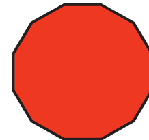
Dodecagon
