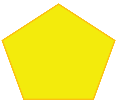
Pentagon
